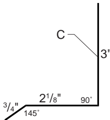
BASE TRIM 402DC with 1 1/2" Hat Channel
