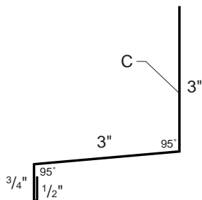
BASE TRIM 402DC with 1 1/2" Hat Channel
