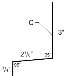
BASE TRIM 168DC-2 with 7/8" Hat Channel
